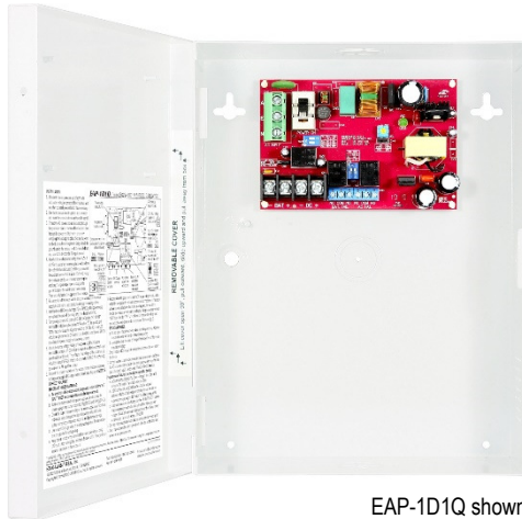
EAP-1D1Q shown
