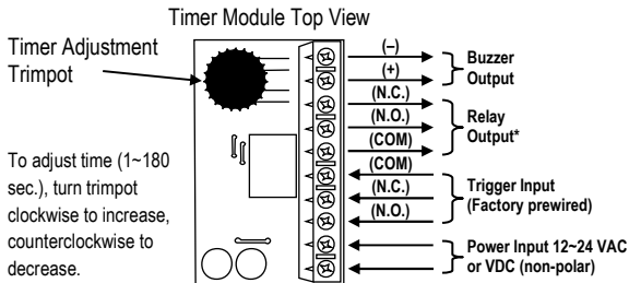
Figure 3 – Timer Outputs (SD-7103GC-PTQ only)
