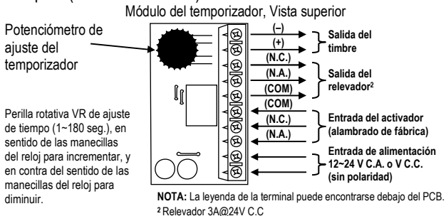
Figure 3 – Timer Outputs (SD-7103GC-PTQ)
