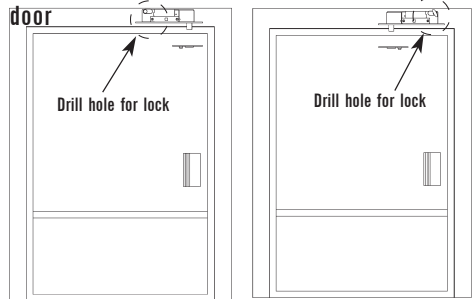
Installation at top of door
