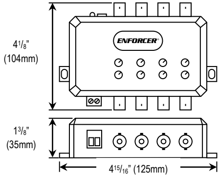
VA-2404B-WQ VA-2404B-WAQ
